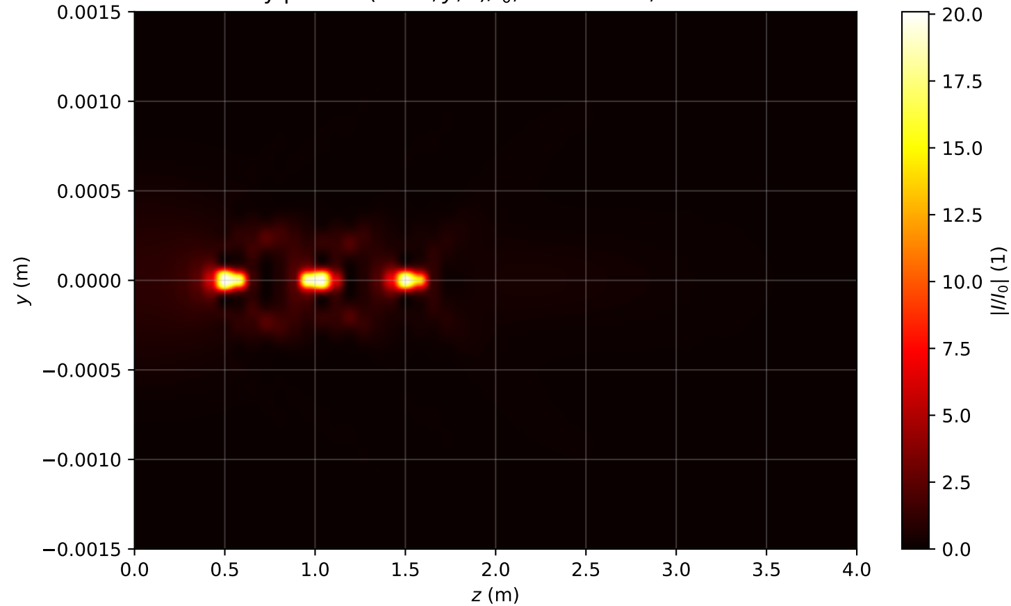
Intensity profile I(x=0, y, z)/I_0 , P_{in}=5.5P_{cr} , artificial time
